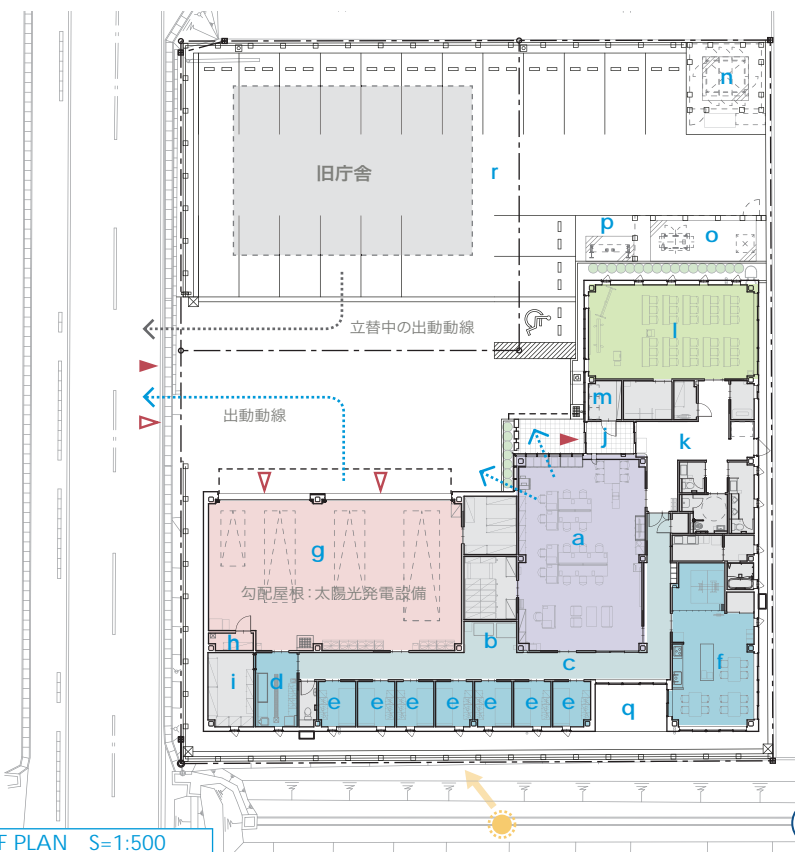
1F PLAN S=1:500
